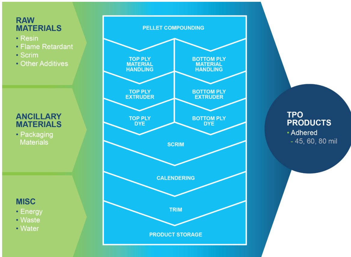
FIGURE 1 Process Flow Diagram of TPO Manufacturing
